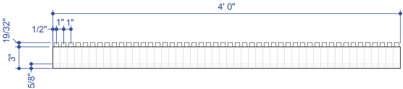
Height Adjuster - Front View
