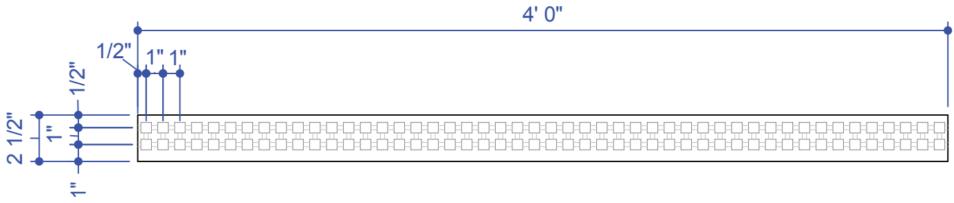
Height Adjuster - Top View
