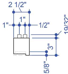
A 1 Height Adjuster Typical Section
